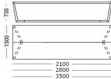
Meeting table with double Top 210x130 cm 280x130 cm 350x130 cm
