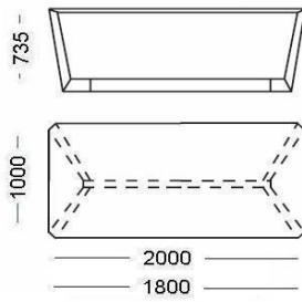
Meeting table with single Top 180x100 cm 200x100 cm
